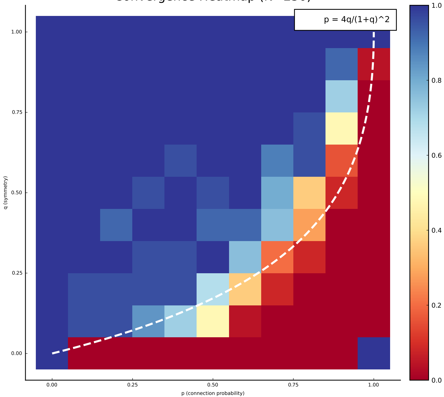
Convergence Heatmap (N=250)
